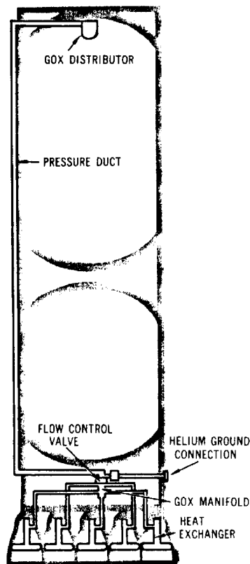
LOX Pressurization
