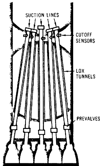
LOX Delivery
