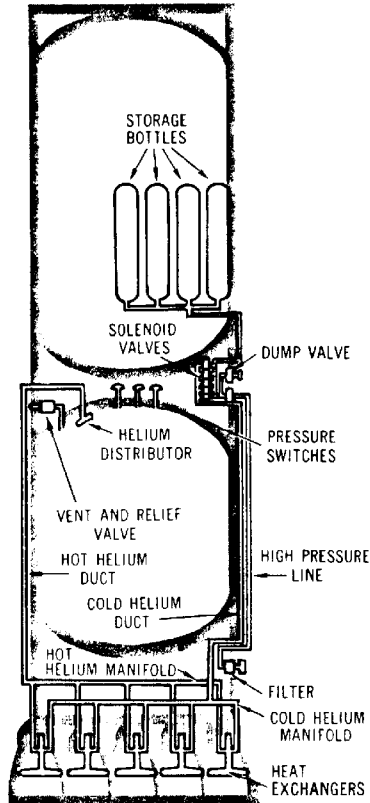
Fuel Pressurization
